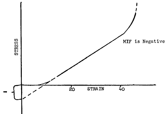
FIG. X3.3 Indentation Stress-Strain Curve (MIF is negative)
